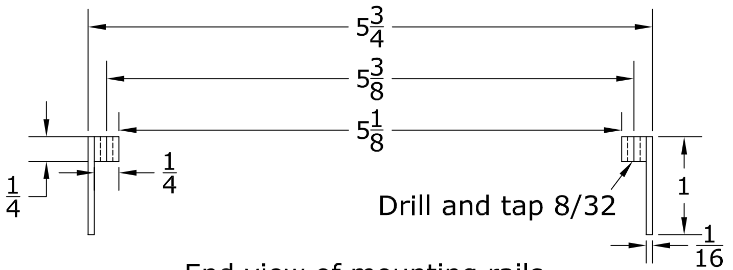
End view of mounting rails
